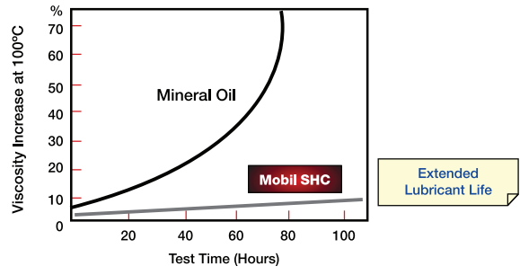
Comparison of Mobil SHC versus a mineral oil in oxidation stability testing.
